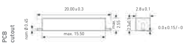
PMC-1001ZHL
