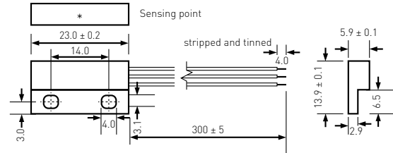
TS-324R
