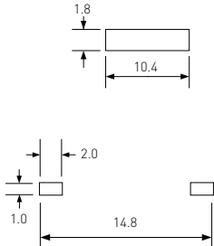
PMC-1001ZHL
