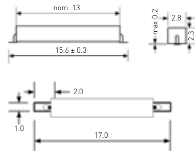
PMC-1001FH
