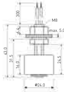
PLS-031 – Miniature
