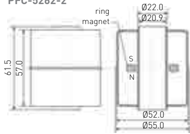
PFC-5262-2
