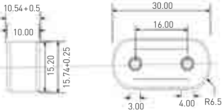
PFC-5262-2
