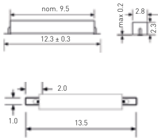
PMC-0701FH
