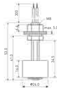
PLS-041 – Standard
