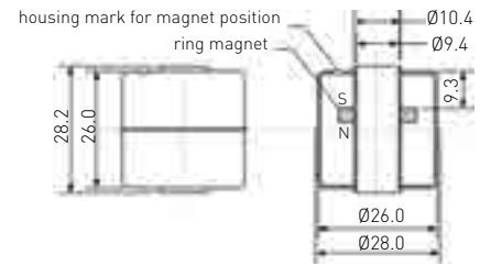
PFC-2828-2
