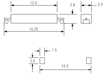
PMC1401THX
