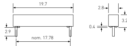
MS-107
