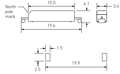
PMC1401THX
